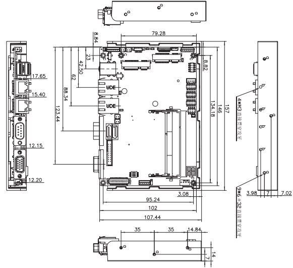
WAFER-ULT2-i1/WAFER-ULT-i1
